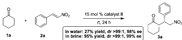
Scheme 2. Michael Reaction in Aqueous Medium
