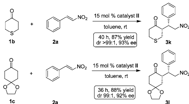
Scheme 1. Different Ketones Reacted with trans -Nitrostyrene
