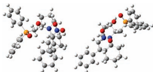
Figure 2. DFT-calculated transition state TS1 (left) and TS2 (right).
