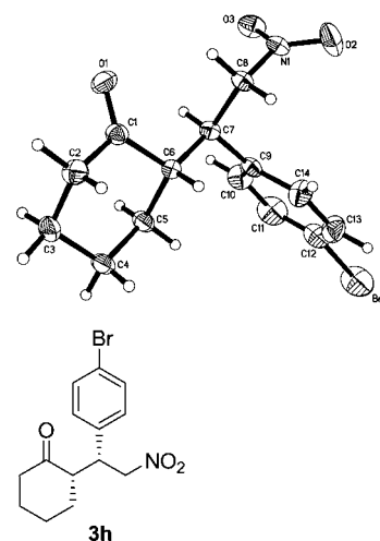
Figure 3. X-ray crystal structure of 3h .
